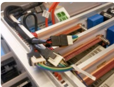
Fig. 4. 12V, direct connection.
